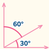
Complementary The two add to 90^\circ
