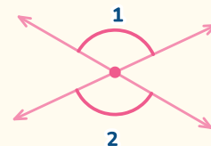
Vertical angles Opposite, and equal
