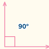
Right angle Exactly 90^\circ
