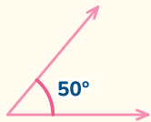
Acute angle Less than 90^\circ
