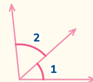
Adjacent angles A shared side
