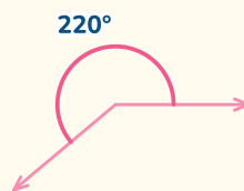
Reflex angle More than 180^\circ
